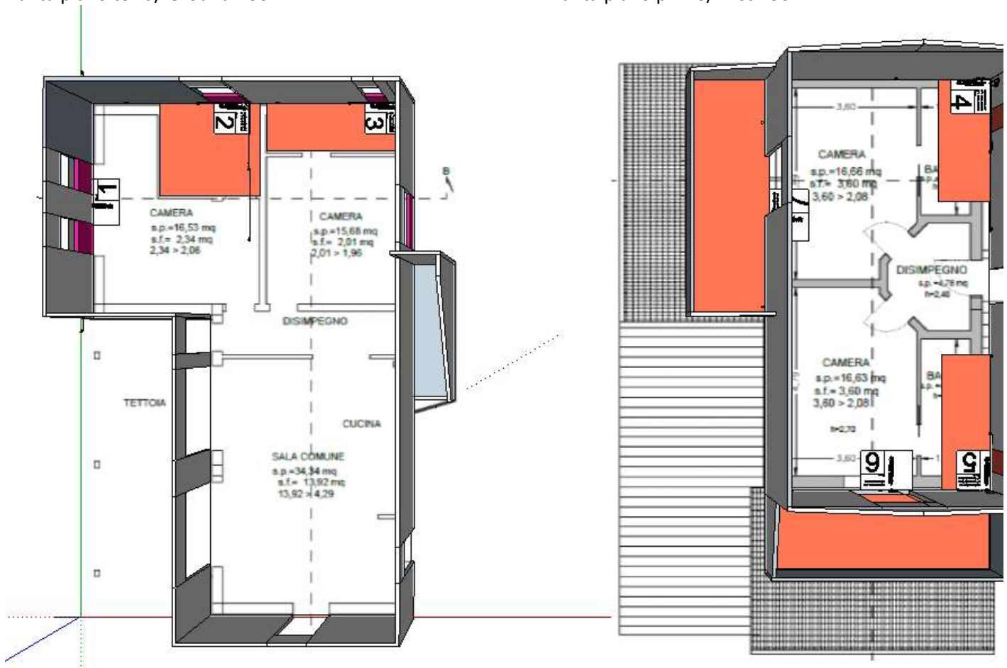
Pianta piano terra/ Ground floor
